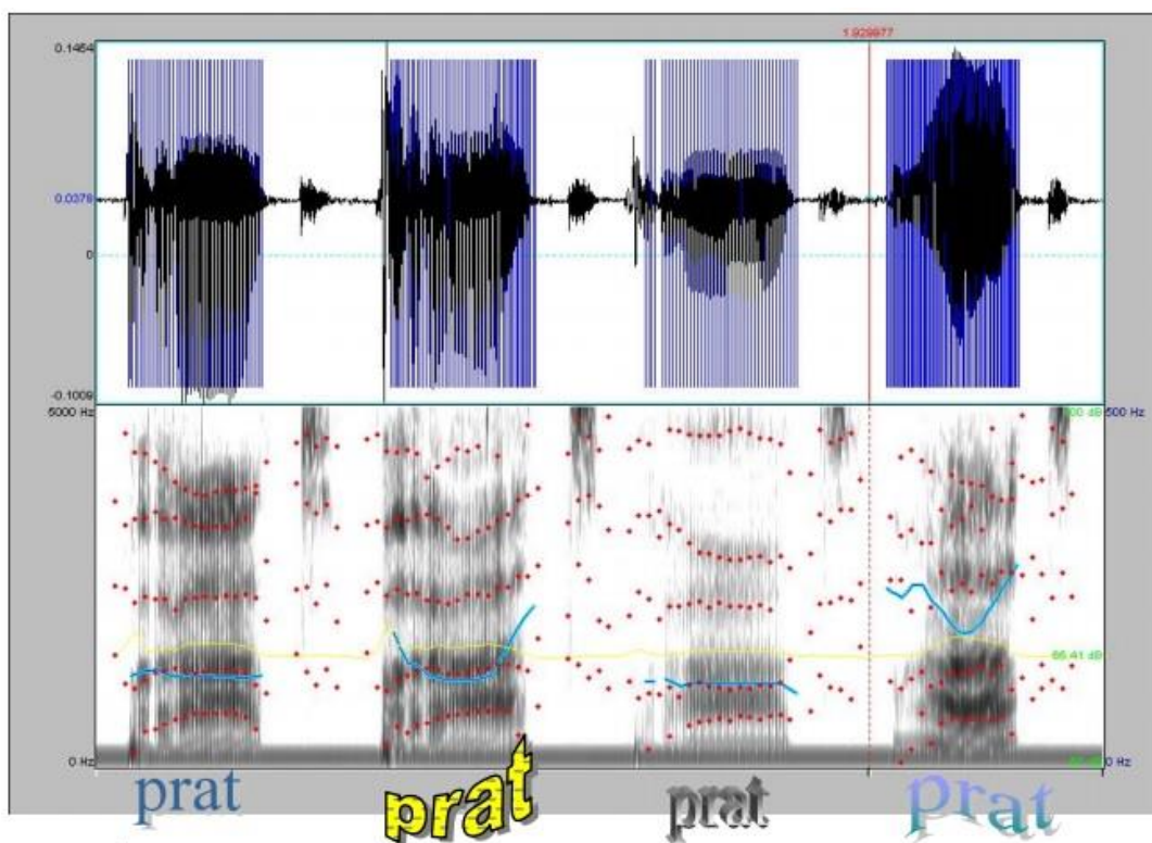
Slika 7. Prikaz spektrograma (donji redak) i oscilograma (gornji redak) (Preuzeto iz https://web.stanford.edu/dept/linguistics/corpora/material/PRAAT_workshop_manual_v421.pdf ).
